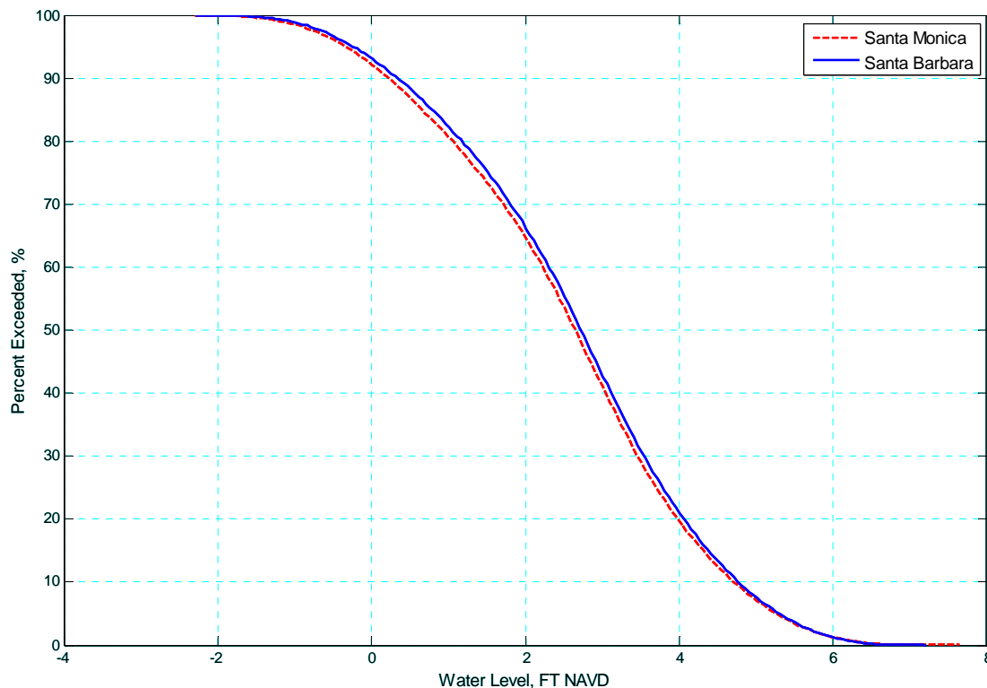
Figure A.6. Water level frequency of exceedance.
