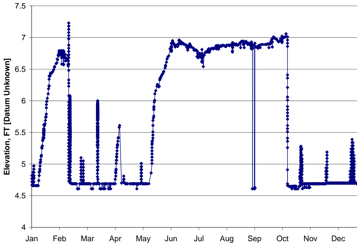
Figure 5.7. J Street 793 Alert Gage stage data for 2003.
