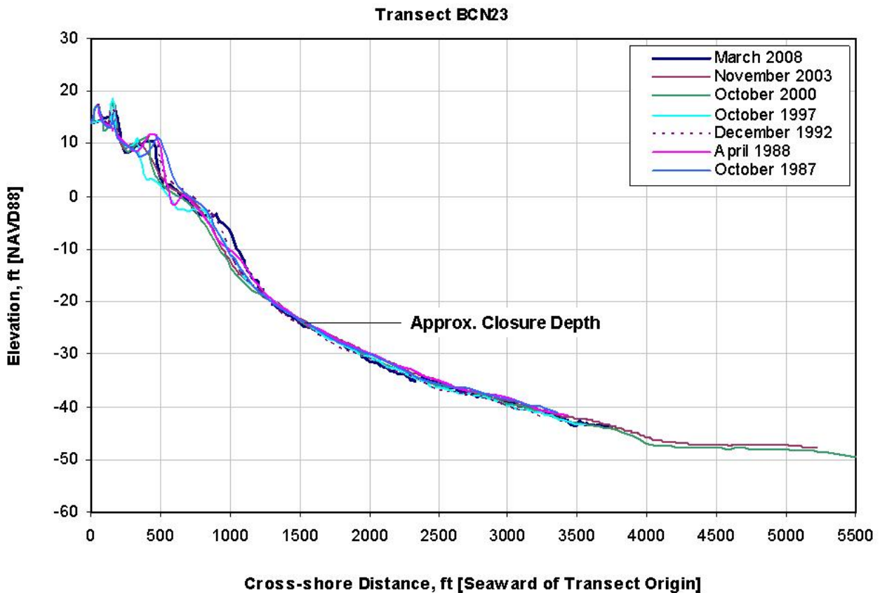
Figure 5.2. Historical cross-shore profiles for Transect BCN23.
