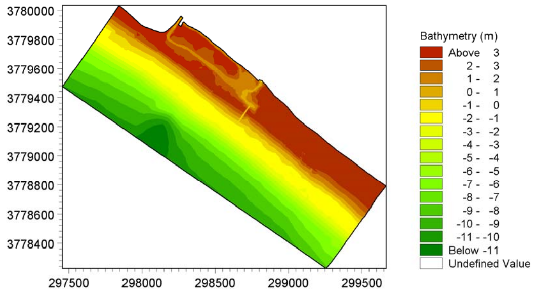
Figure B.3 - Breaching Model Domain, emergency mechanical breach near OID.
