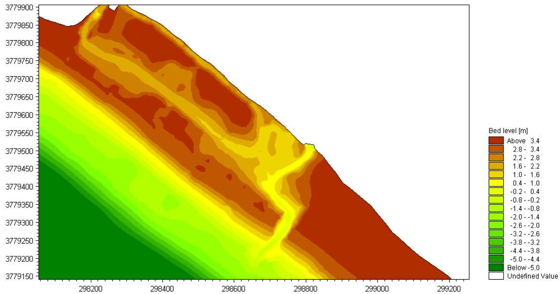
Figure B.21. Bed level after the 2 year storm with an inlet near OID.
