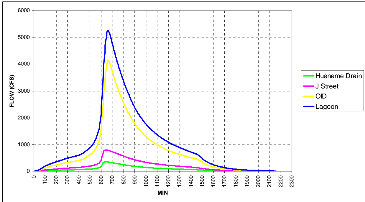
Figure 5.11. Hydrograph for 100-year event.
