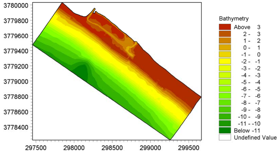
Figure B.2 - Breaching Model Domain, maintained beach.
