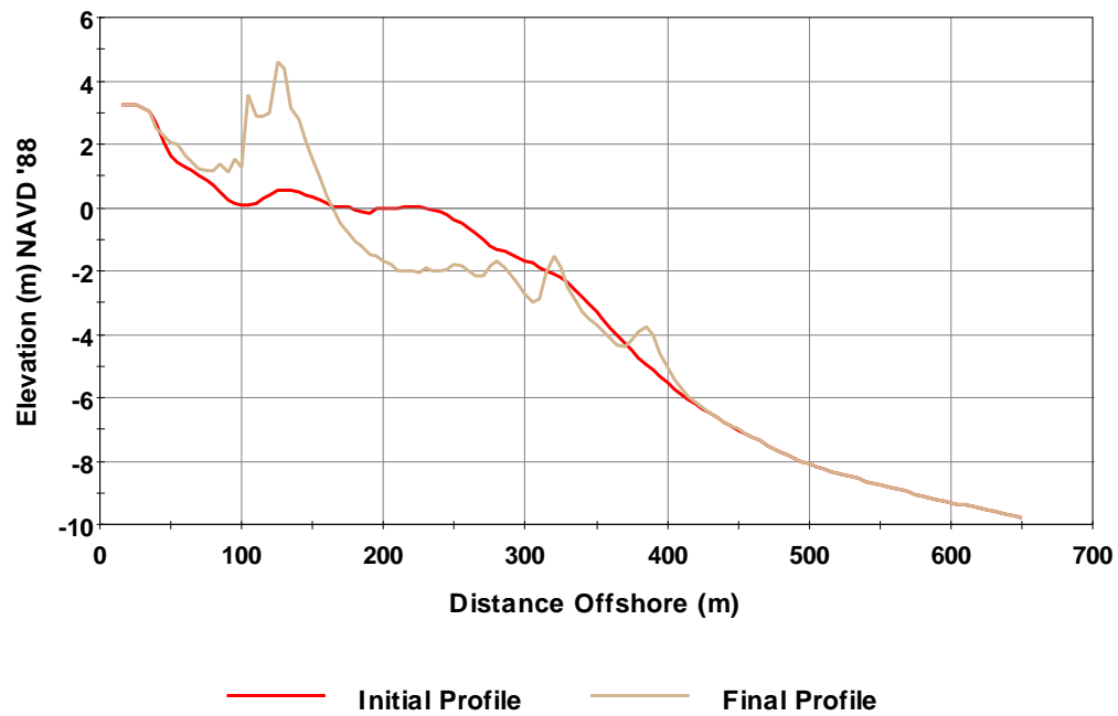
Figure B.26. Modeled cross-shore profile change, February 20 – March 20, 2008
