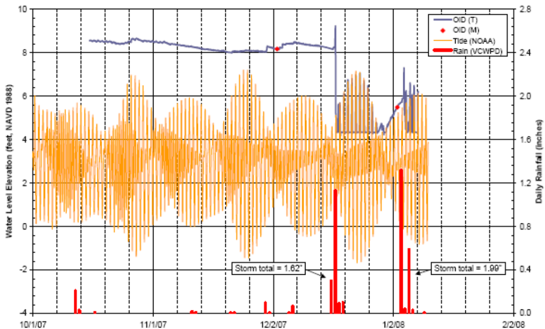
Figure 5.9. Water level in the lagoon 10/2007 – 1/2008 (CH2M Hill 2008).
