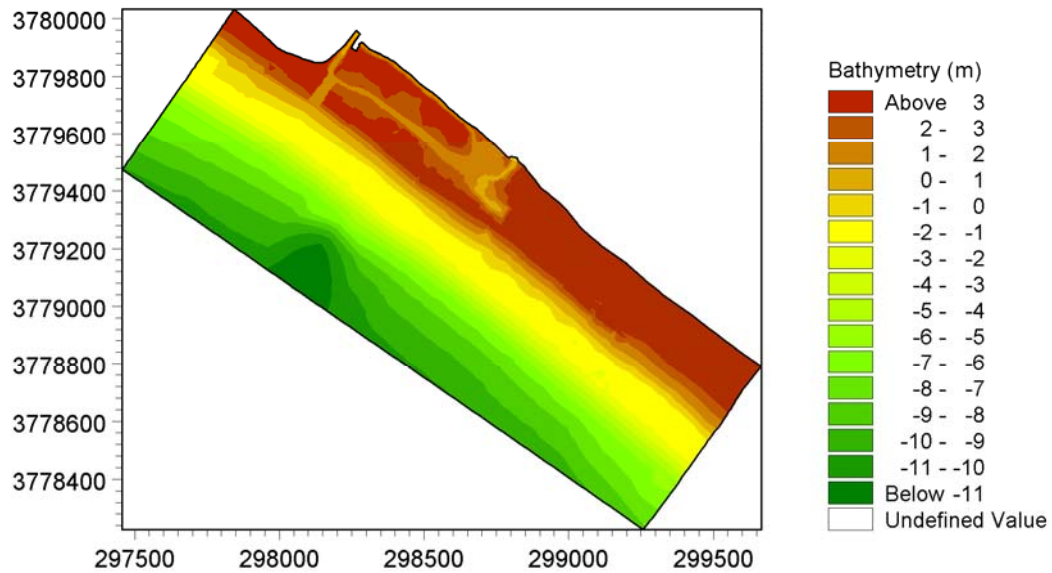
Figure B.4 – Breaching model domain, emergency mechanical breach near J Street.
