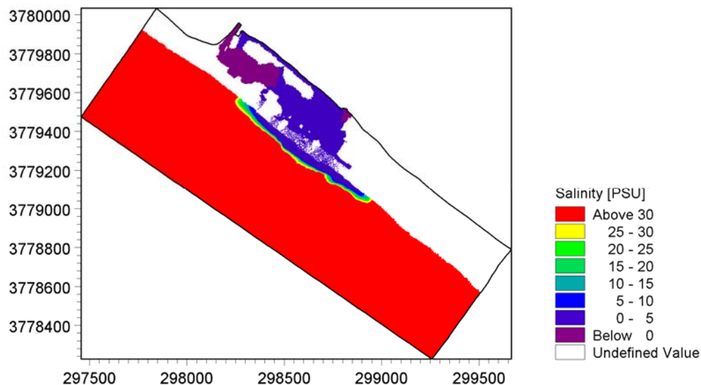
Figure B.12. Salinity at 2-year peak flow over idealized representative beach.
