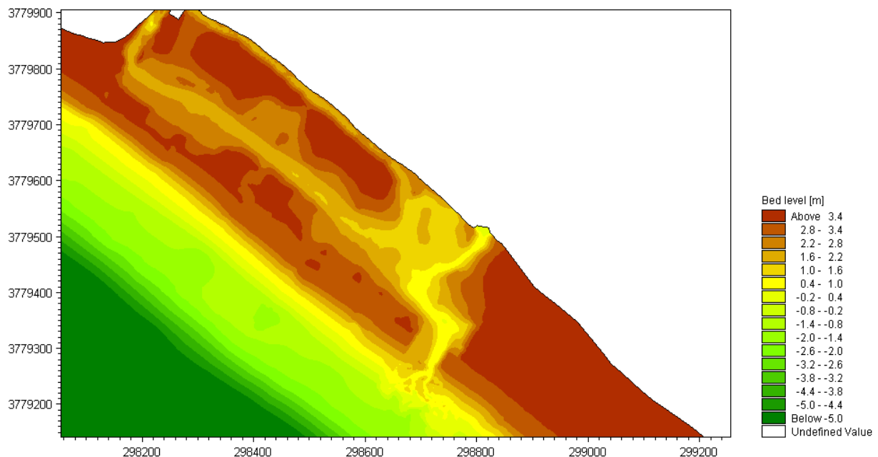
Figure B.17. Bed level at the end of the 2 year storm over the maintained beach.
