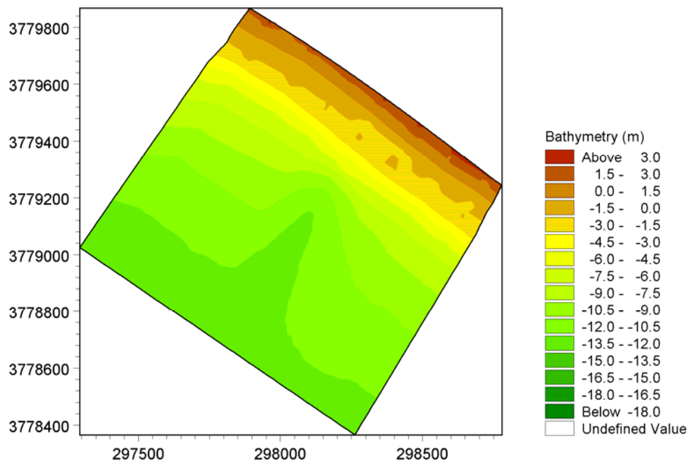
Figure B.5 – Calibration Model Domain.
