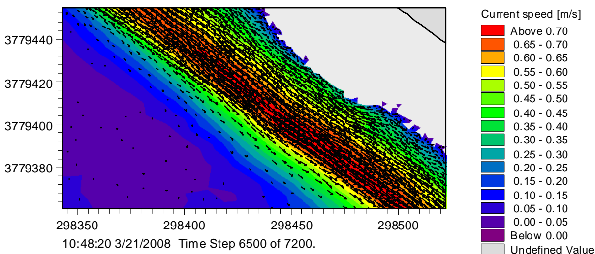
Figure B.9 – Enlarged wave and tide induced currents during model verification.
