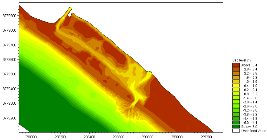
Figure B.23. Bed level after the 100 year storm with an inlet near OID.
