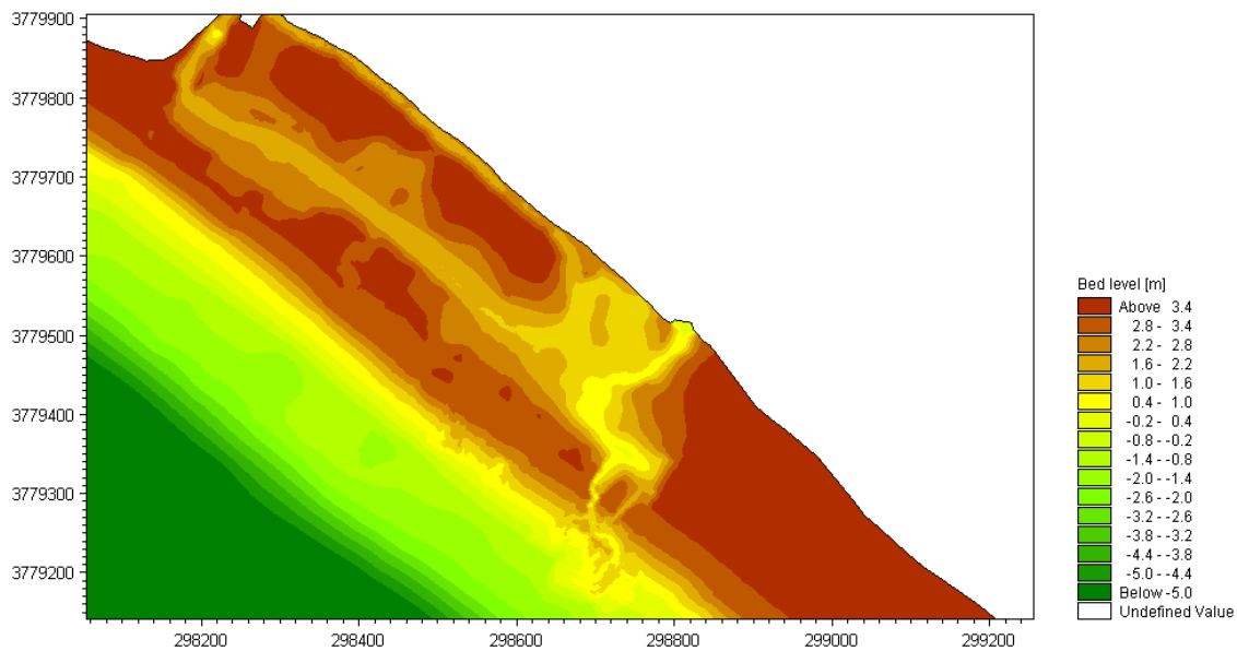
Figure B.14. Bed level at the end of the 2 year storm over the idealized beach.
