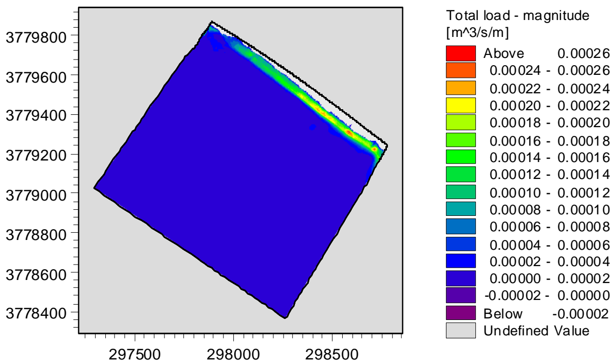
Figure B.10 – Wave and current induced sediment transport during model verification.
