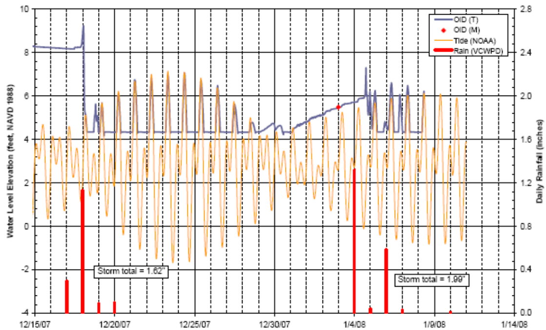
Figure 5.8. Water level in the lagoon 12/5/2007 – 1/10/2008 (CH2M Hill 2008).
