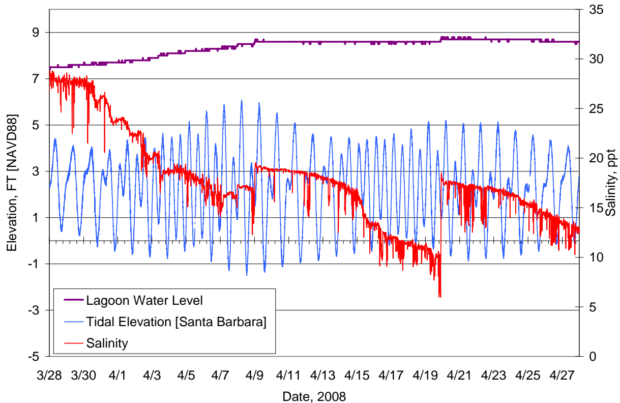
Figure 5.6. Measured lagoon water level, salinity and tide.
