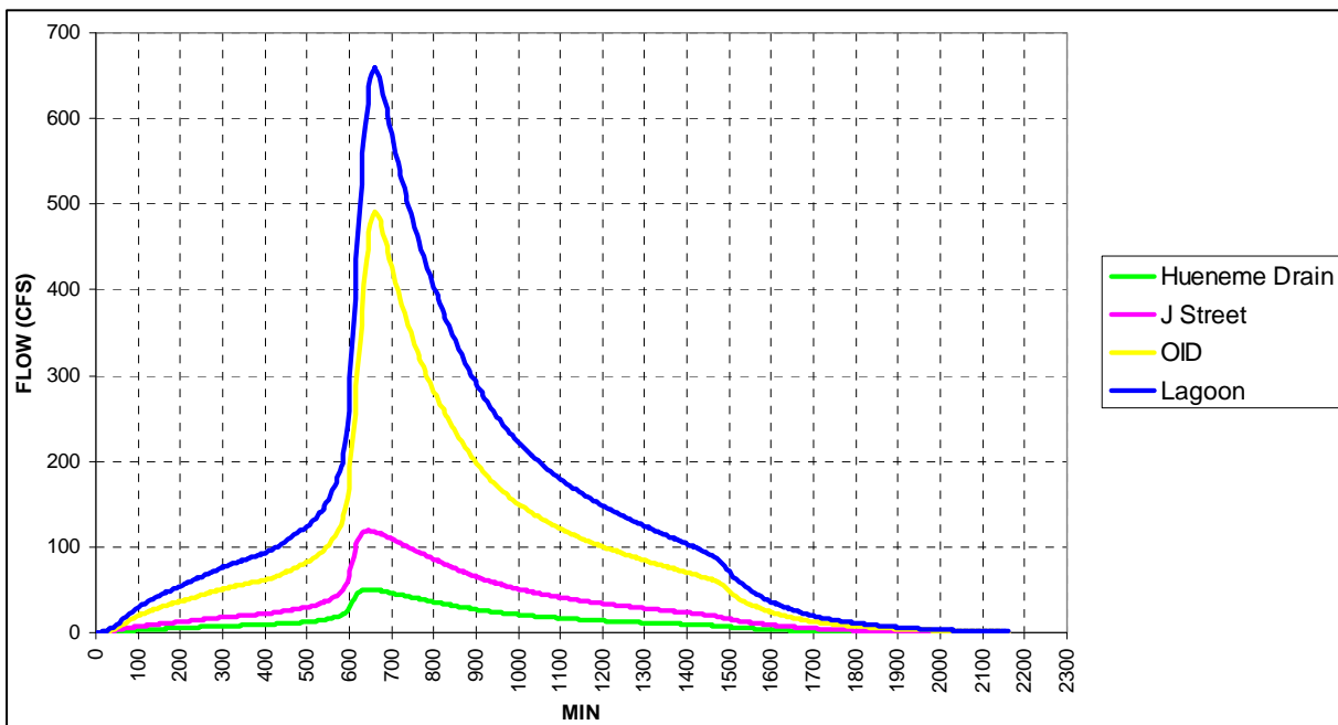
Figure 5.10. Hydrograph for 2-year event.
