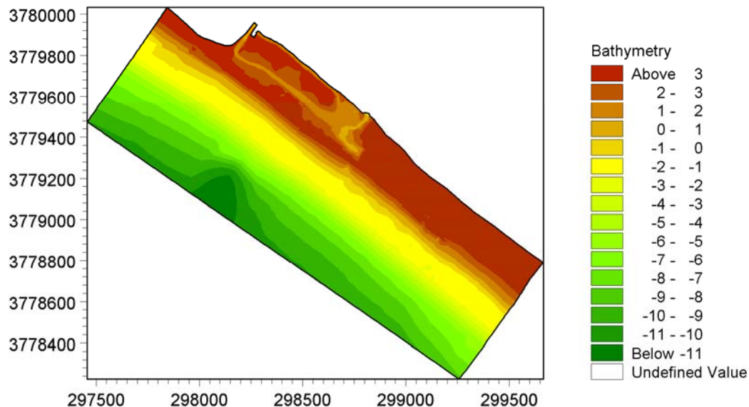
Figure B.1 - Breaching Model Domain, no action idealized beach.
