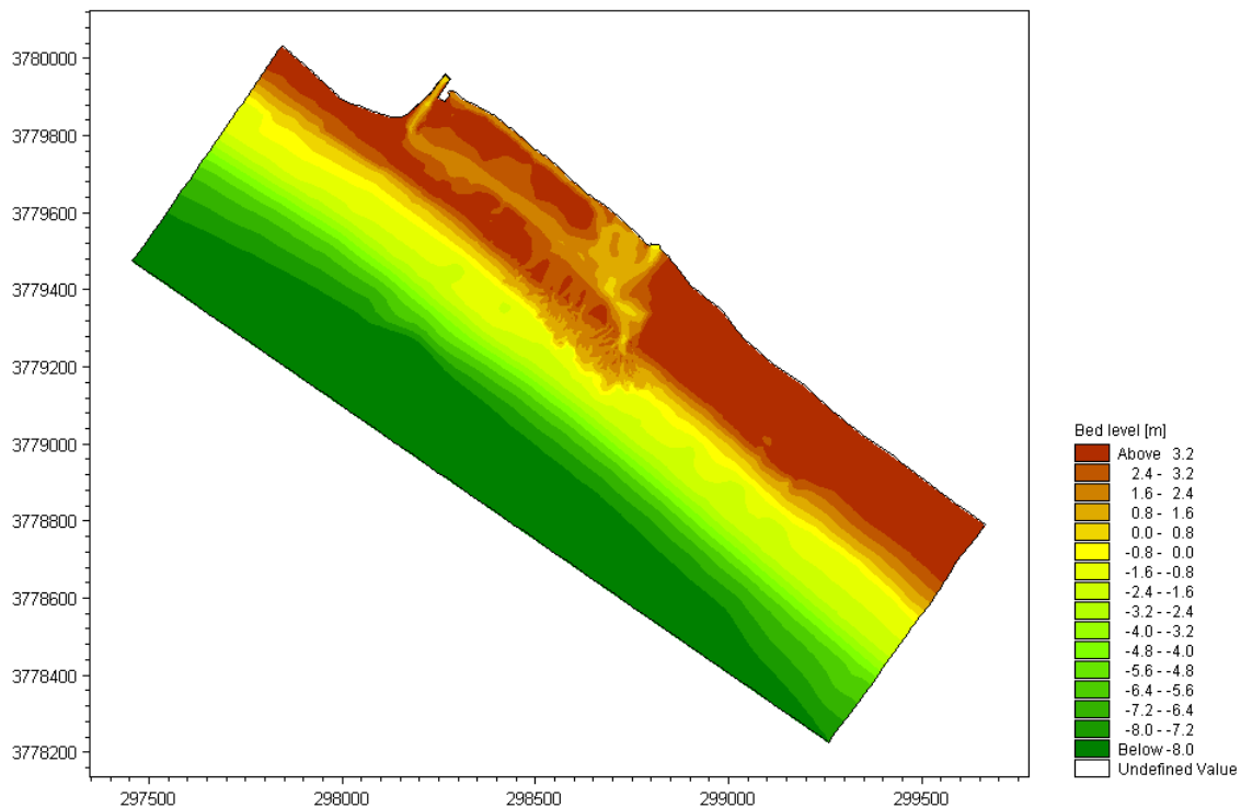
Figure 6.1. Elevation above NAVD at peak flow during the 100-year event.
