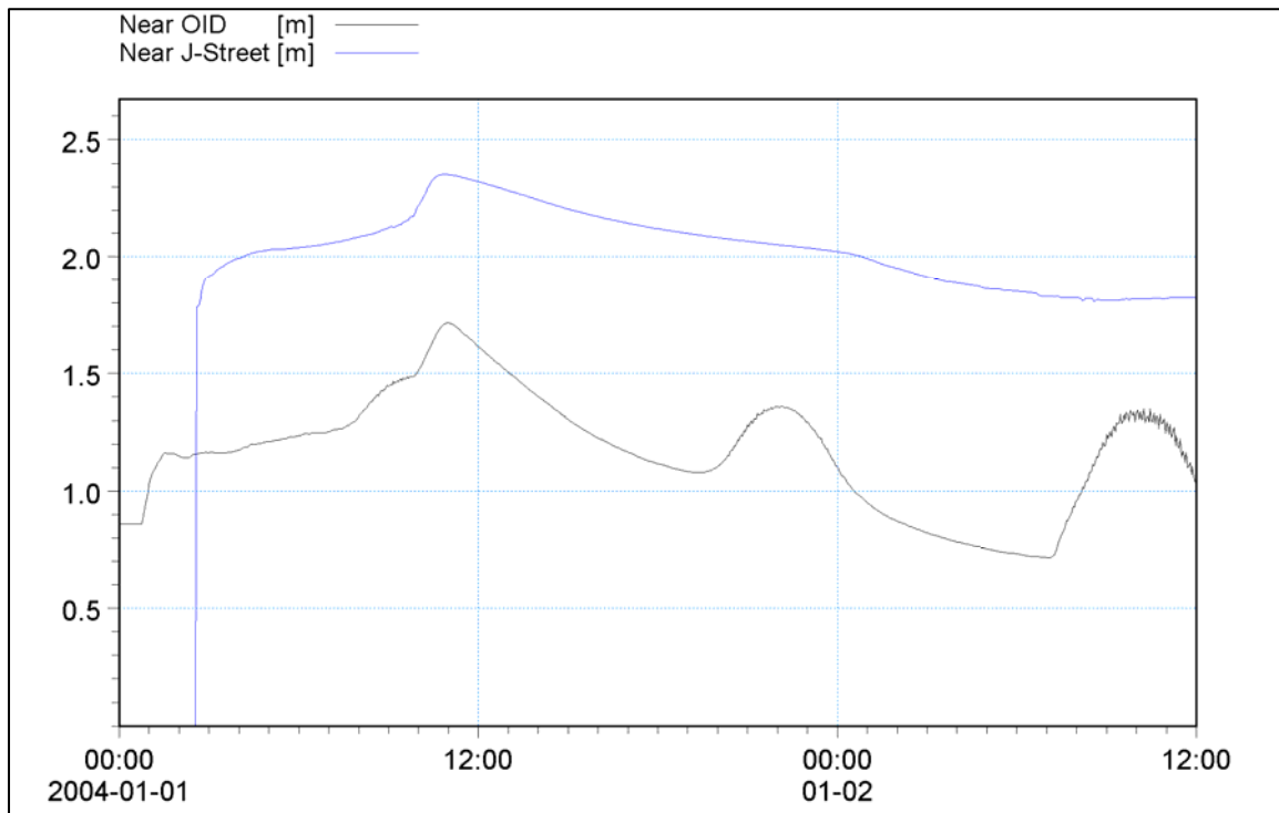
Figure B.19. Water level during the 2-year storm with an emergency breach near OID.
