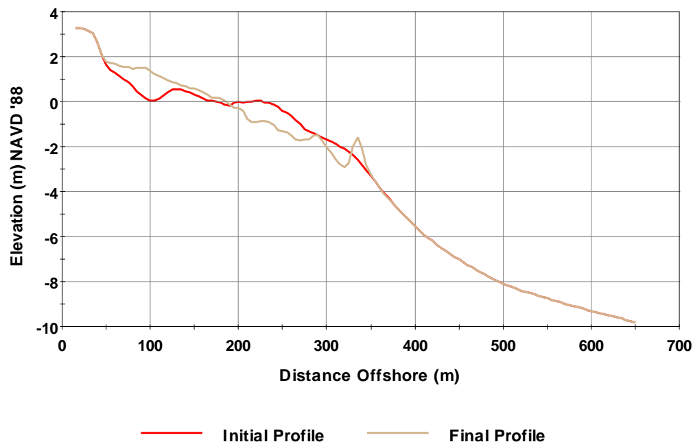
Figure B.25. Modeled cross-shore profile change, March 5 – March 20, 2008
