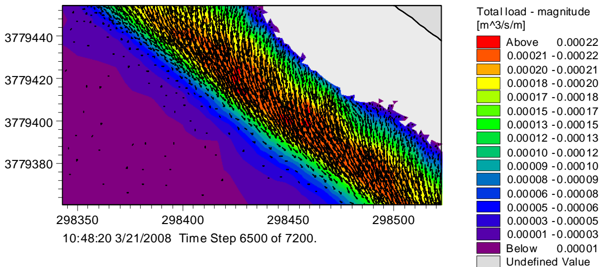
Figure B.11 – Enlarged sediment transport during model verification.
