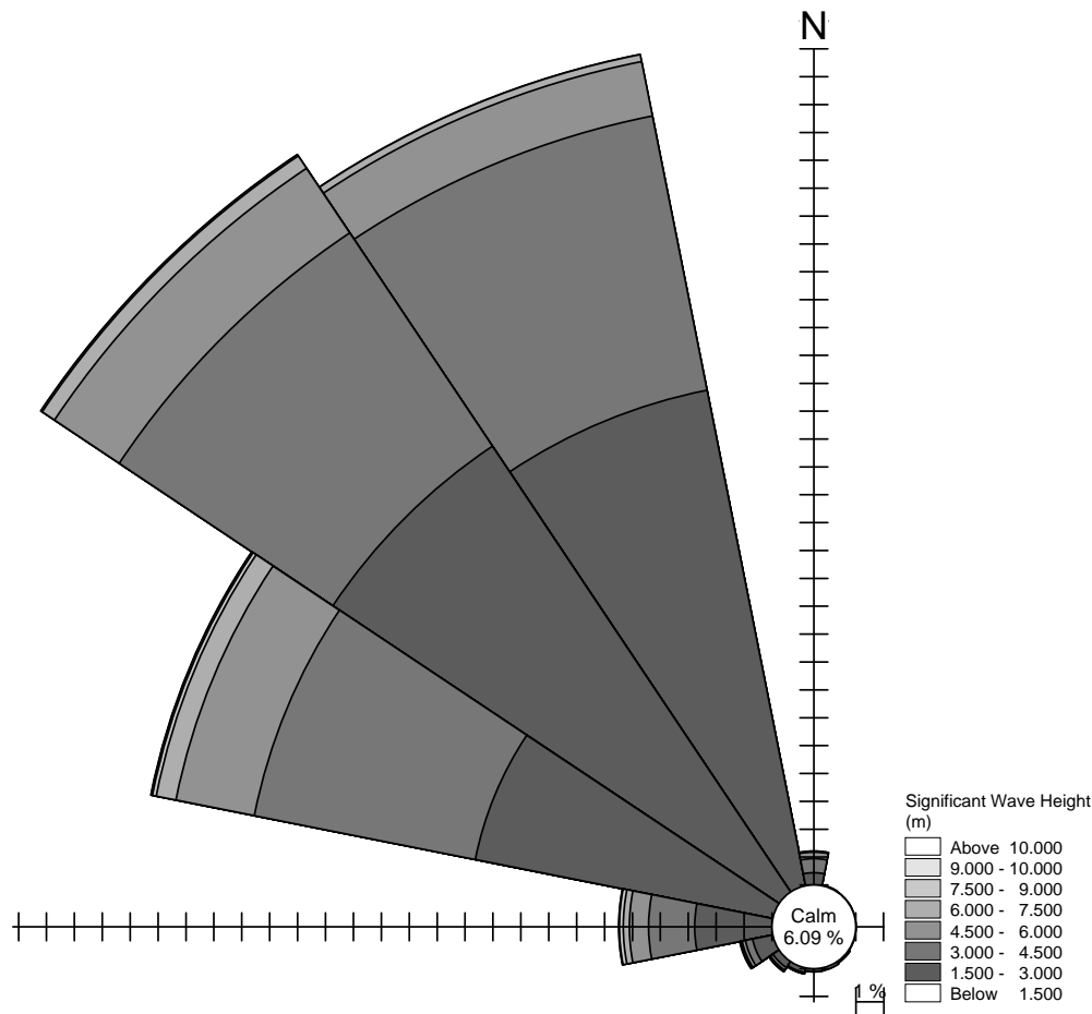
Figure A.5. Wave rose for WIS Station 91.
