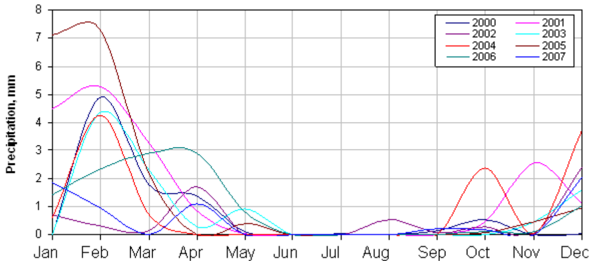
Figure A.7. Monthly precipitation fluctuations in Oxnard, CA.
