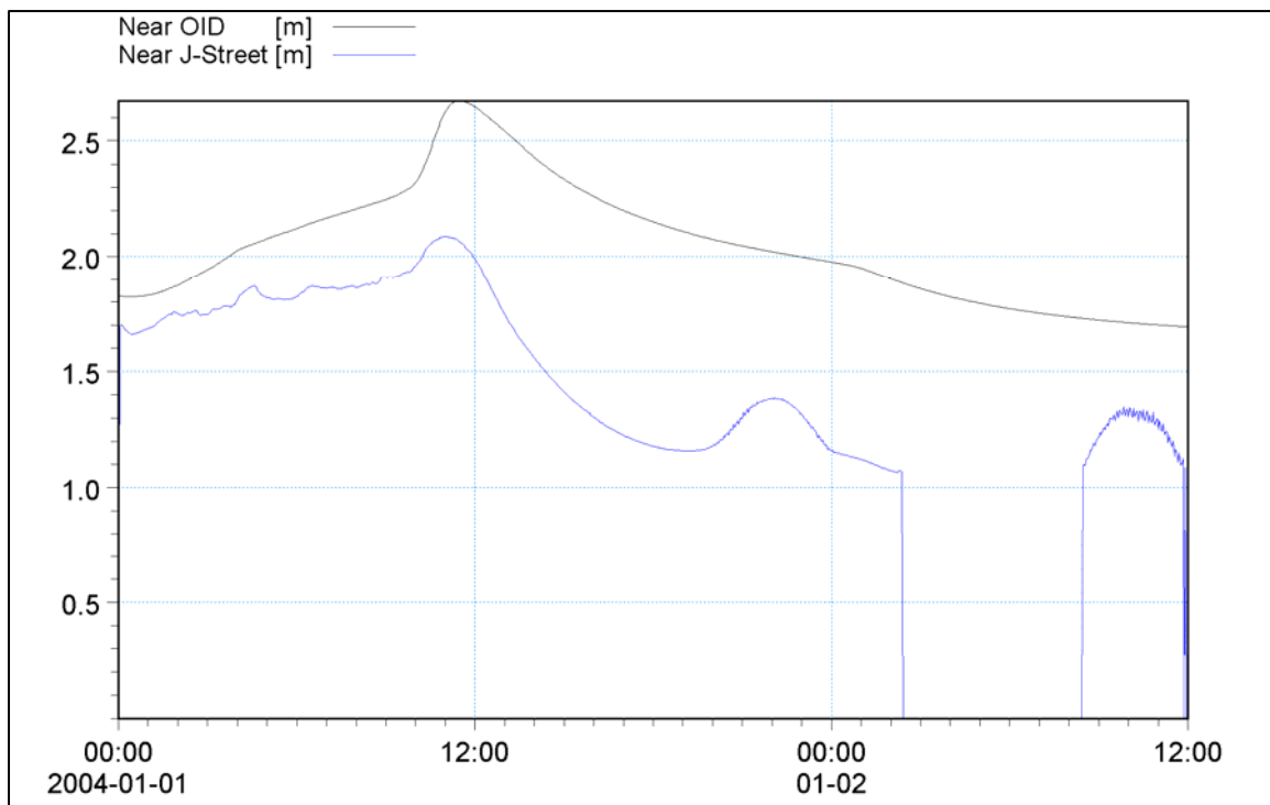
Figure B.20. Water level during the 2 year storm with an inlet near J Street.
