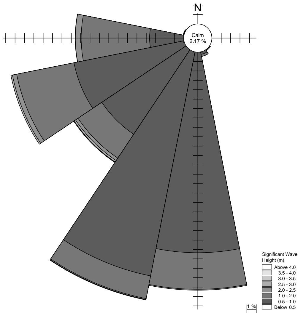
Figure A.4. Wave rose for CDIP Station 141.
