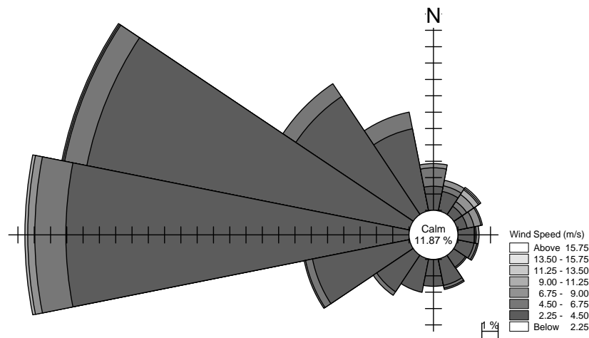
Figure A.3. Wind rose for Port Hueneme.
