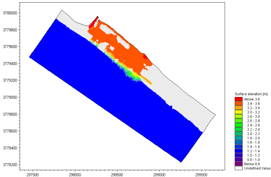
Figure B.16. Peak water level during the 100 year storm over the idealized beach.
