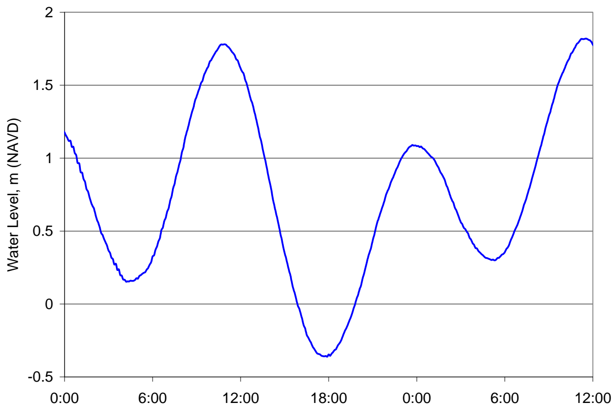
Figure B.6. Water level boundary applied during breaching.
