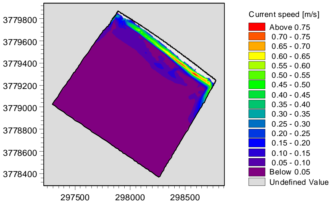
Figure B.8 – Wave and tide induced currents during model verification.
