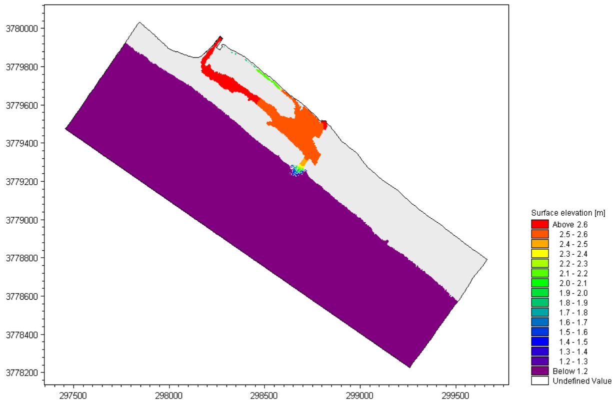
Figure B.18. Peak water level during the 2 year storm over the maintained beach crest.
