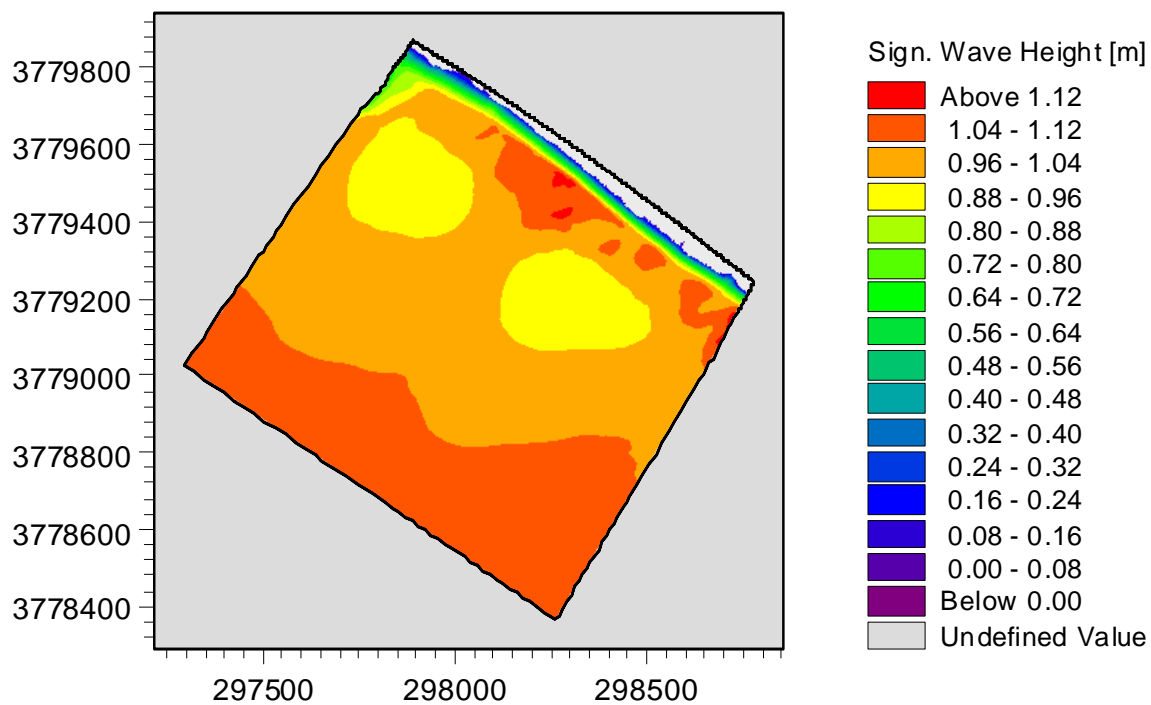
Figure B.7 – Waves during model verification.
