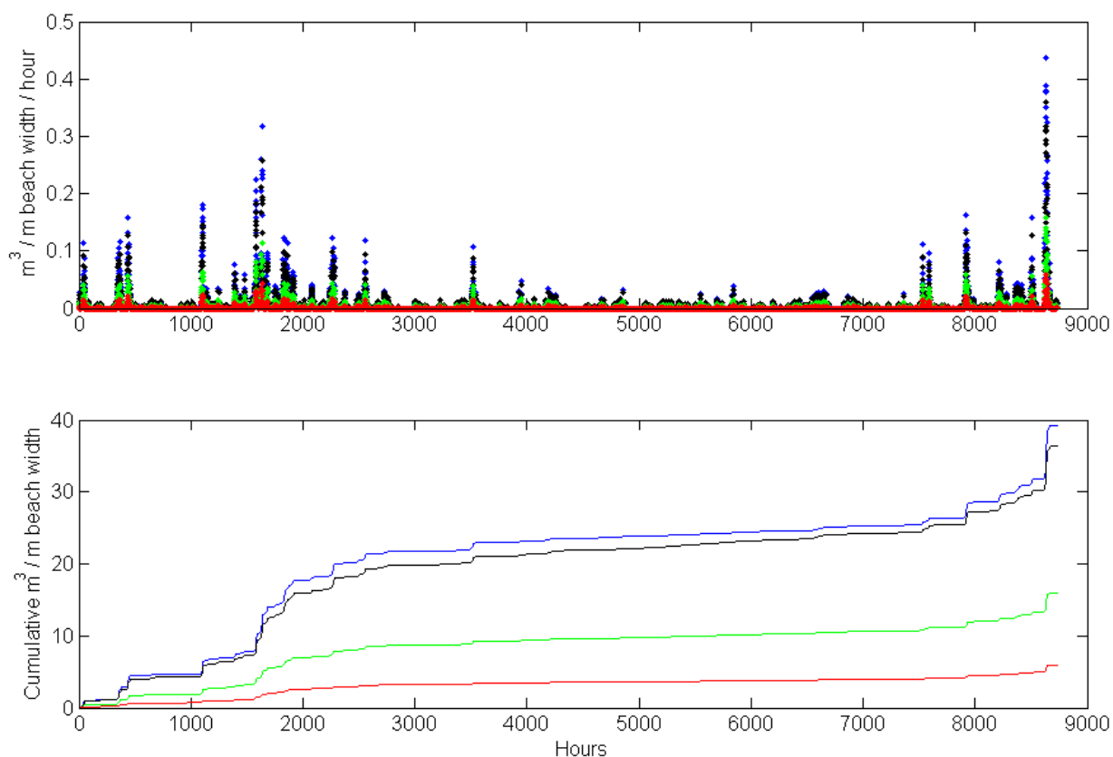
Figure A.8. Four methods for estimating wind-blown sand transport for the year 2006.
