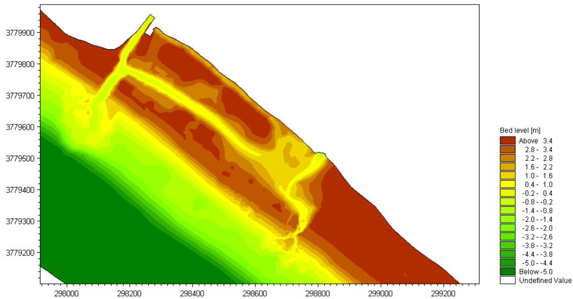
Figure B.24. Bed level after the 100 year storm with an inlet near J-Street.
