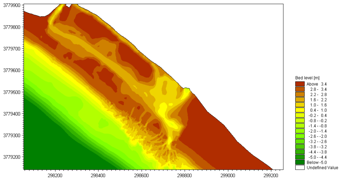
Figure B.15. Bed level at the end of the 100 year storm over the idealized beach.
