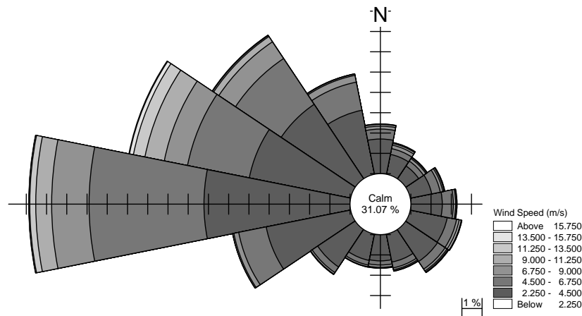
Figure A.2. Wind rose for Santa Monica, Station 46025.
